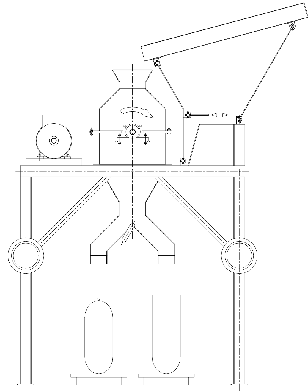
Front View
