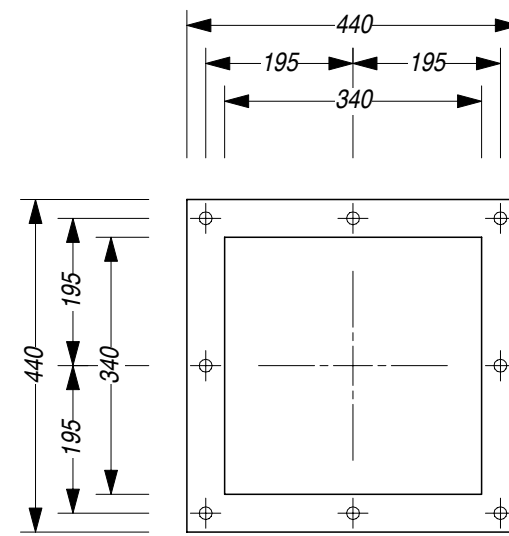
Flange on the Outlet End
