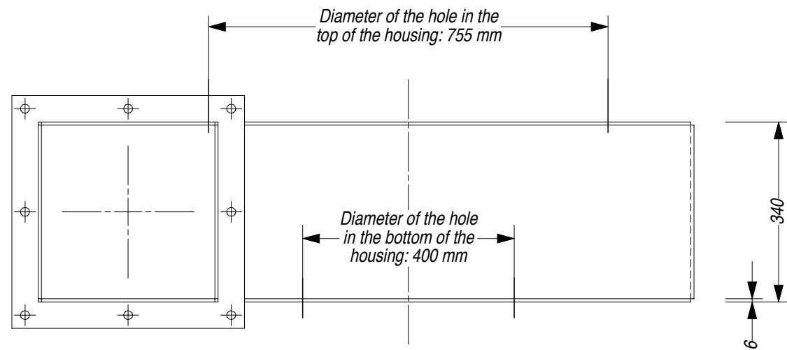
Seen from the Outlet End
