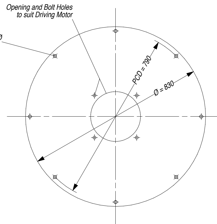
Top Plate - supporting Rotor and Motor (see 3D View above right)
