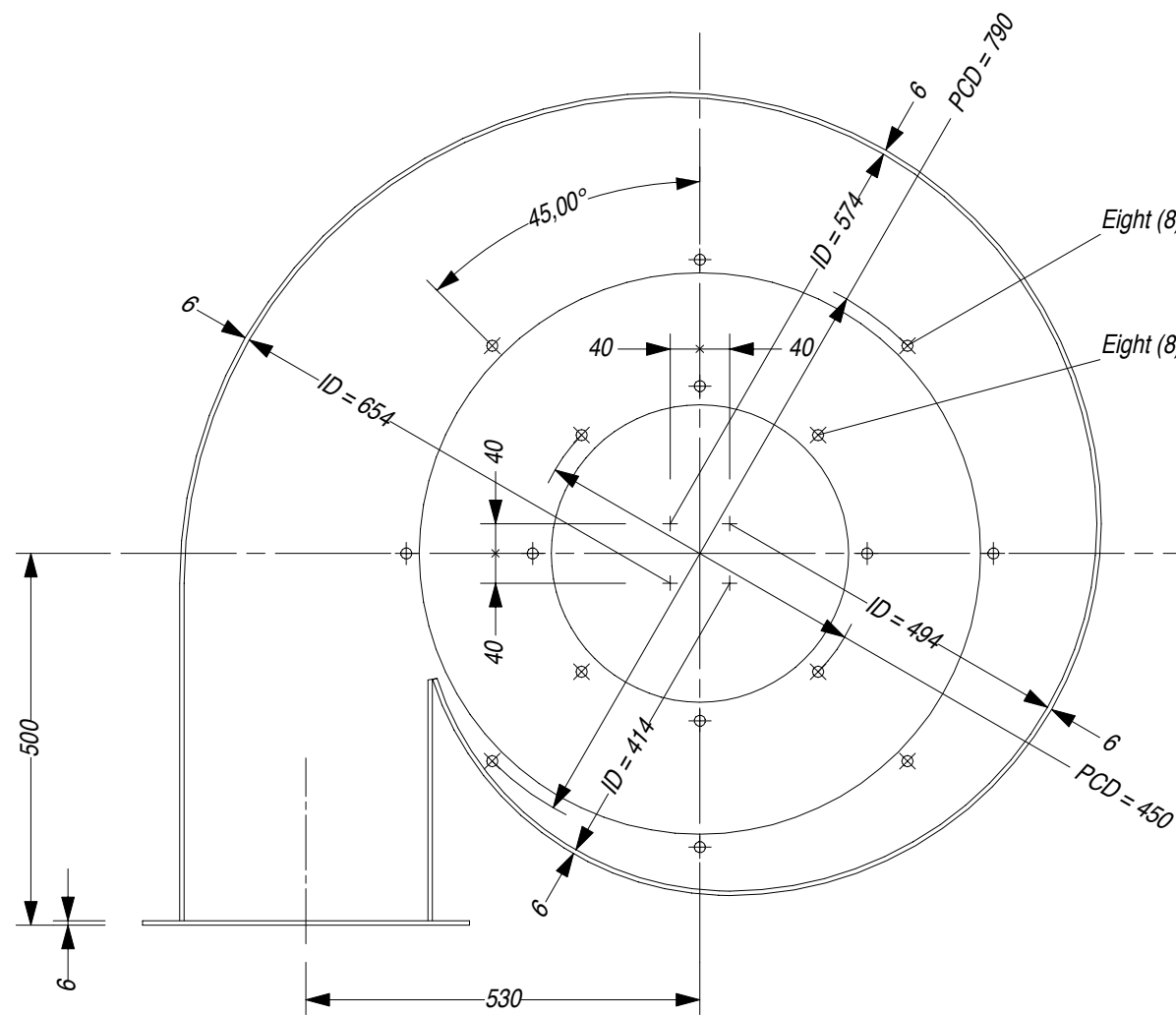
Top / Plan View
